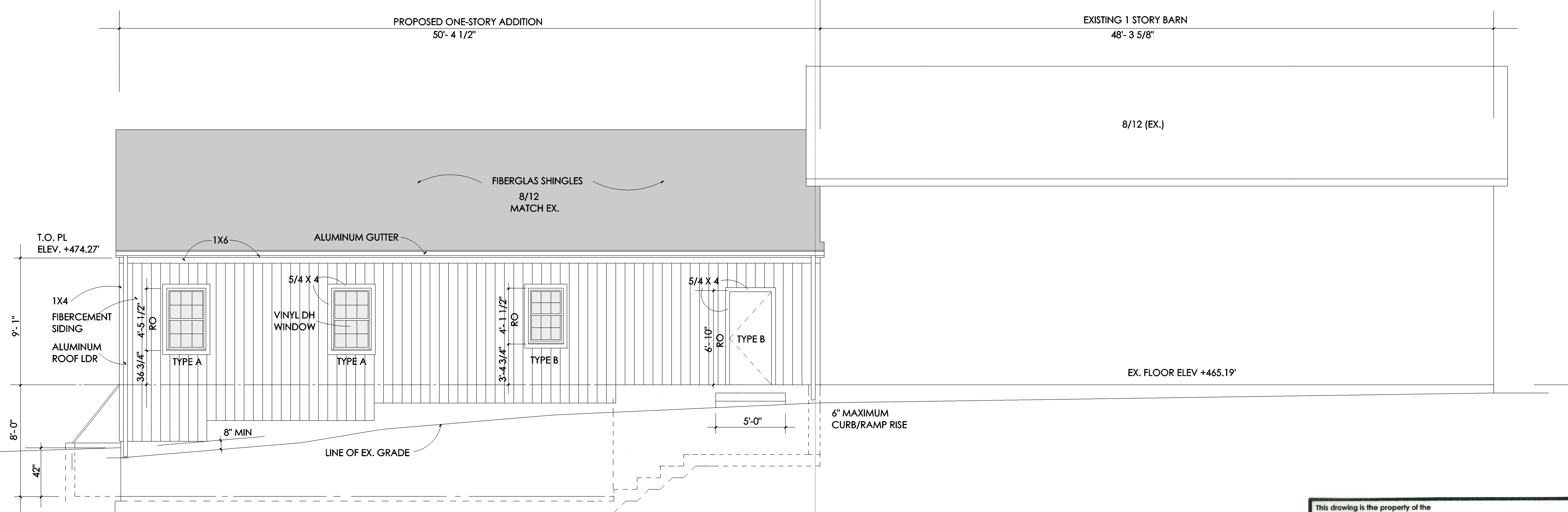
1 NORTH ELEVATION A2 1/4" = 1 FOOT
